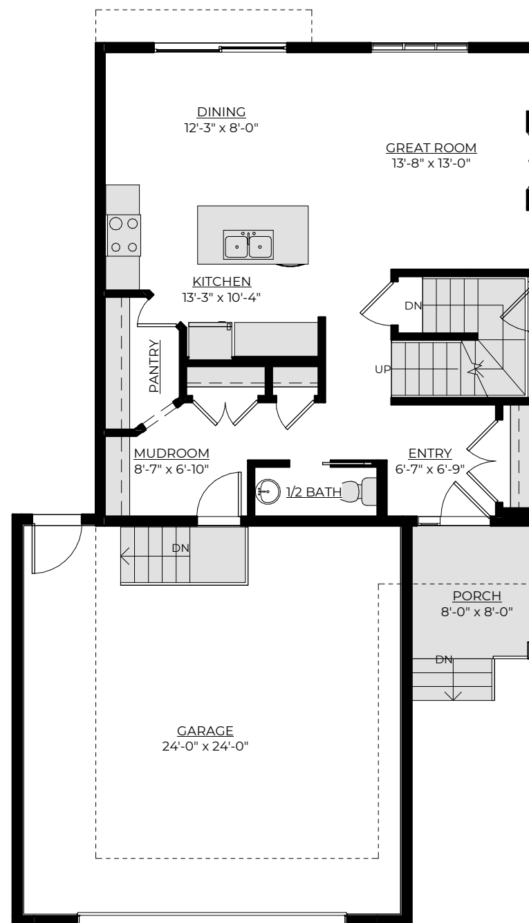
Main Floor Plan 783 ft 2
