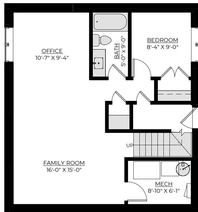
Future Basement Plan 783 ft 2
