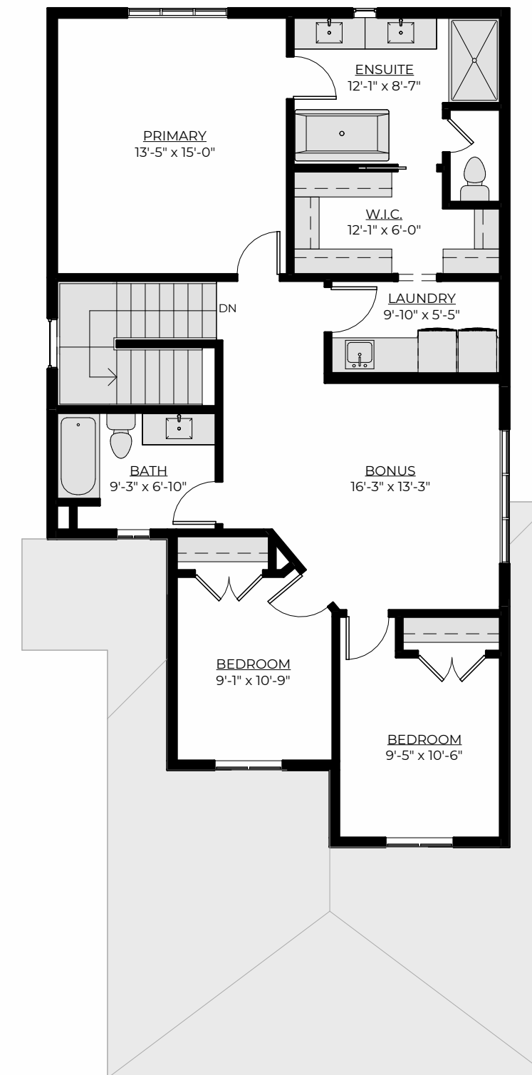
Second Floor Plan Option A 1,155 ft 2
