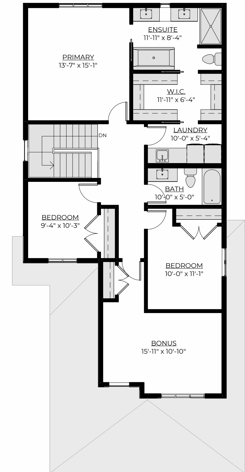
Second Floor Plan Option B 1,229 ft 2
