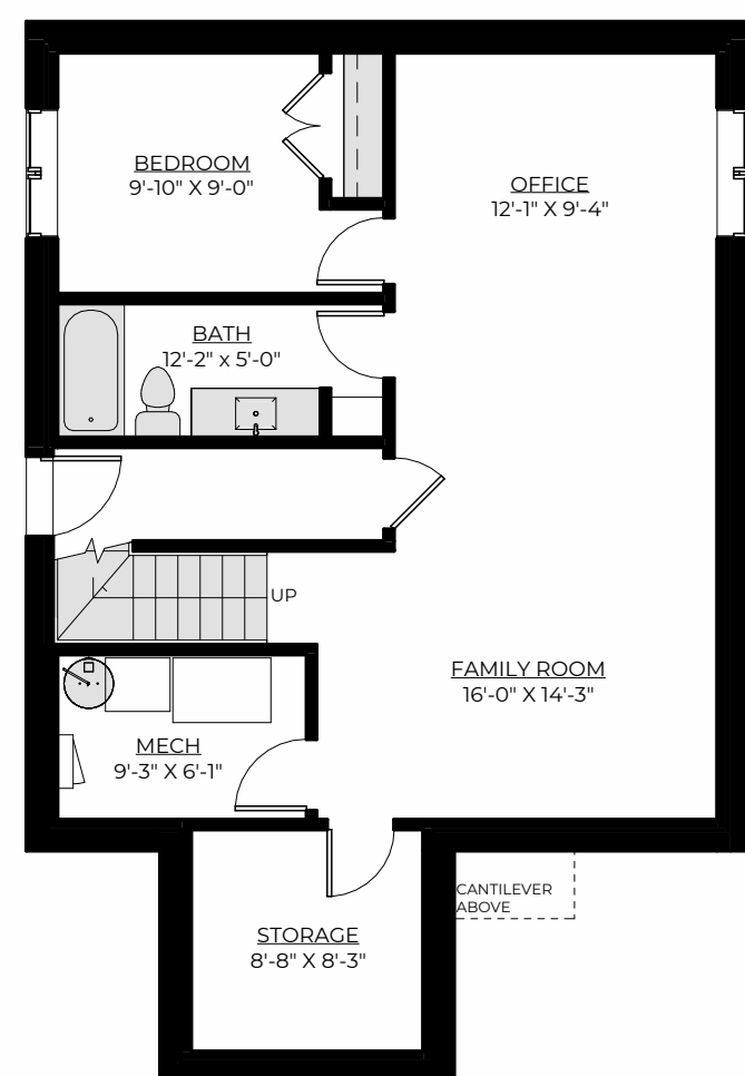
Future Basement Plan 933 ft 2
