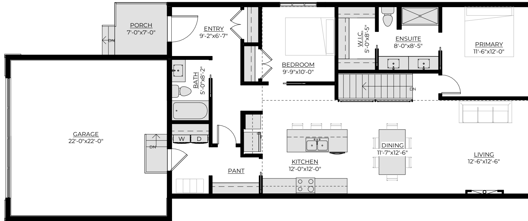
Main Floor Plan 1261 ft 2
