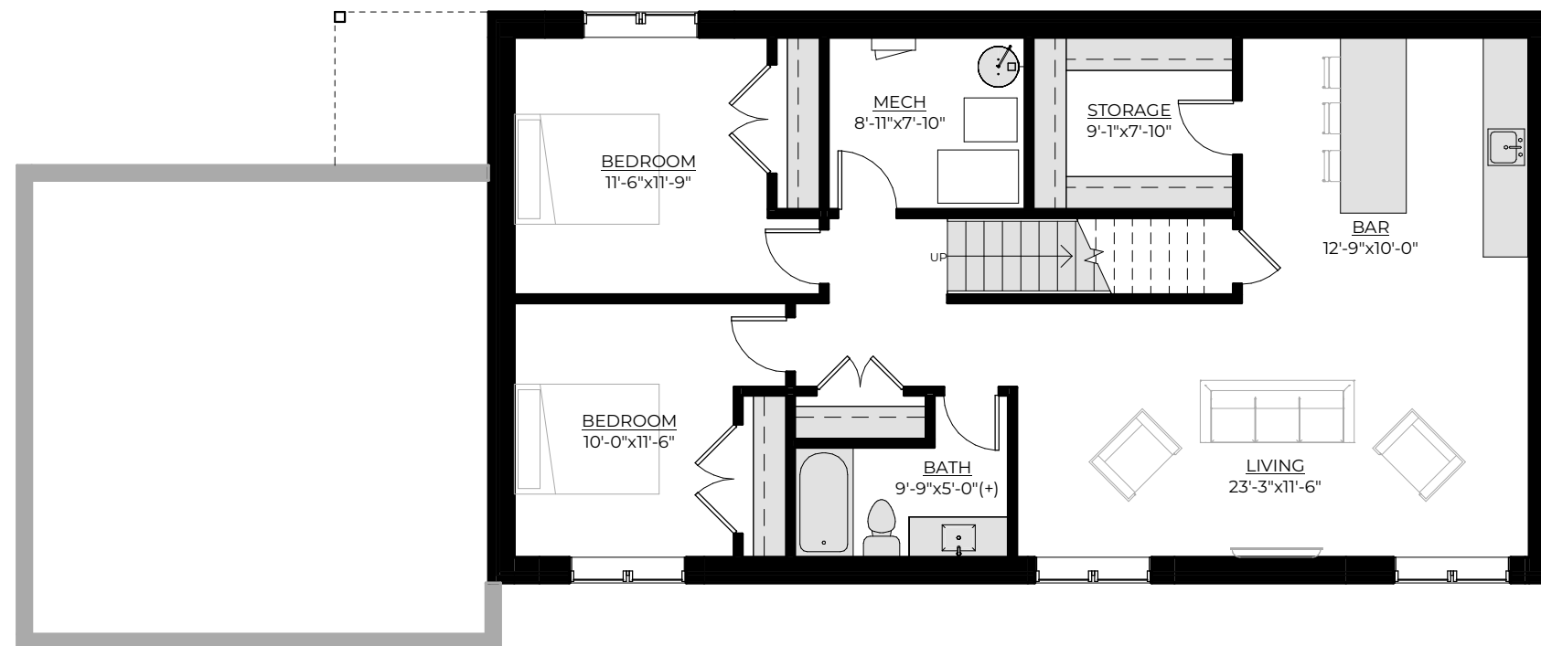
Future Basement Plan 1261 ft 2
