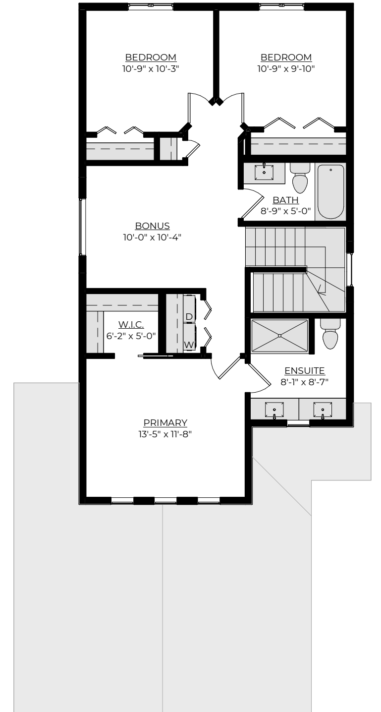
Second Floor Plan 911 ft 2
